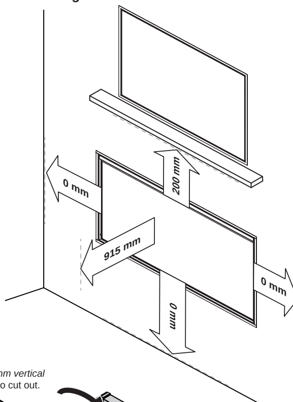
Figure 3. Clearance to Combustibles
