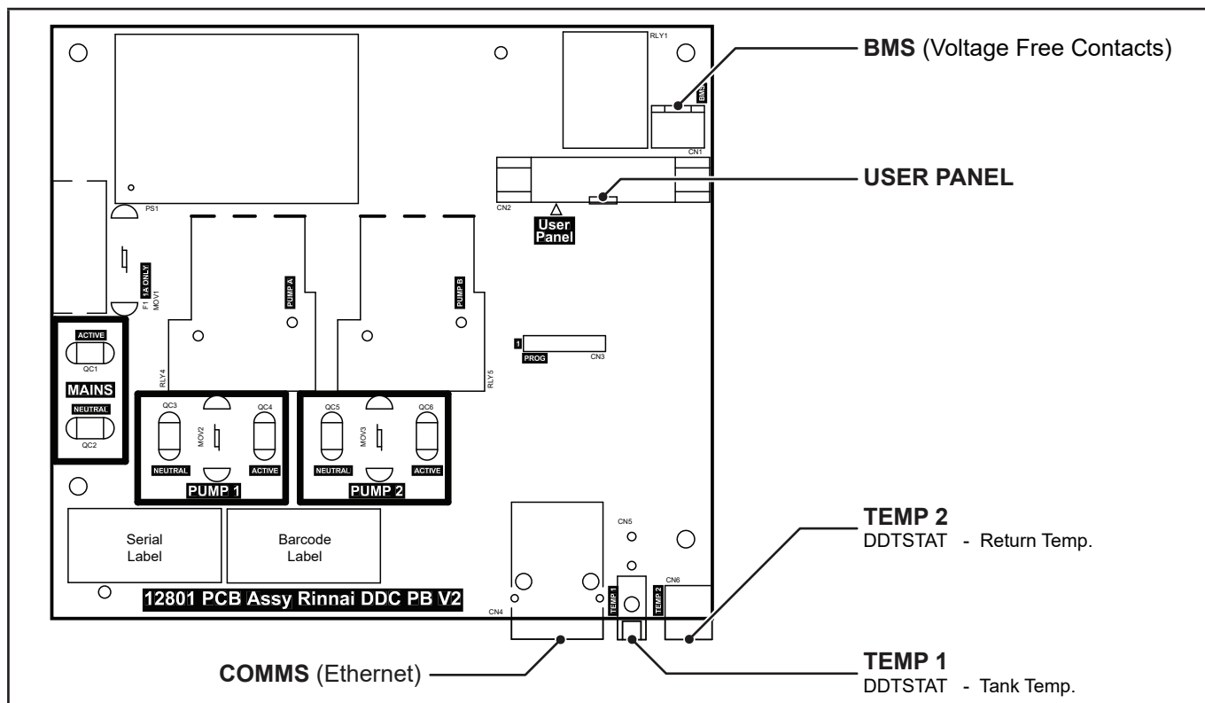
Figure 2. DDSTAT Internal PCB showing Thermistor Connections
