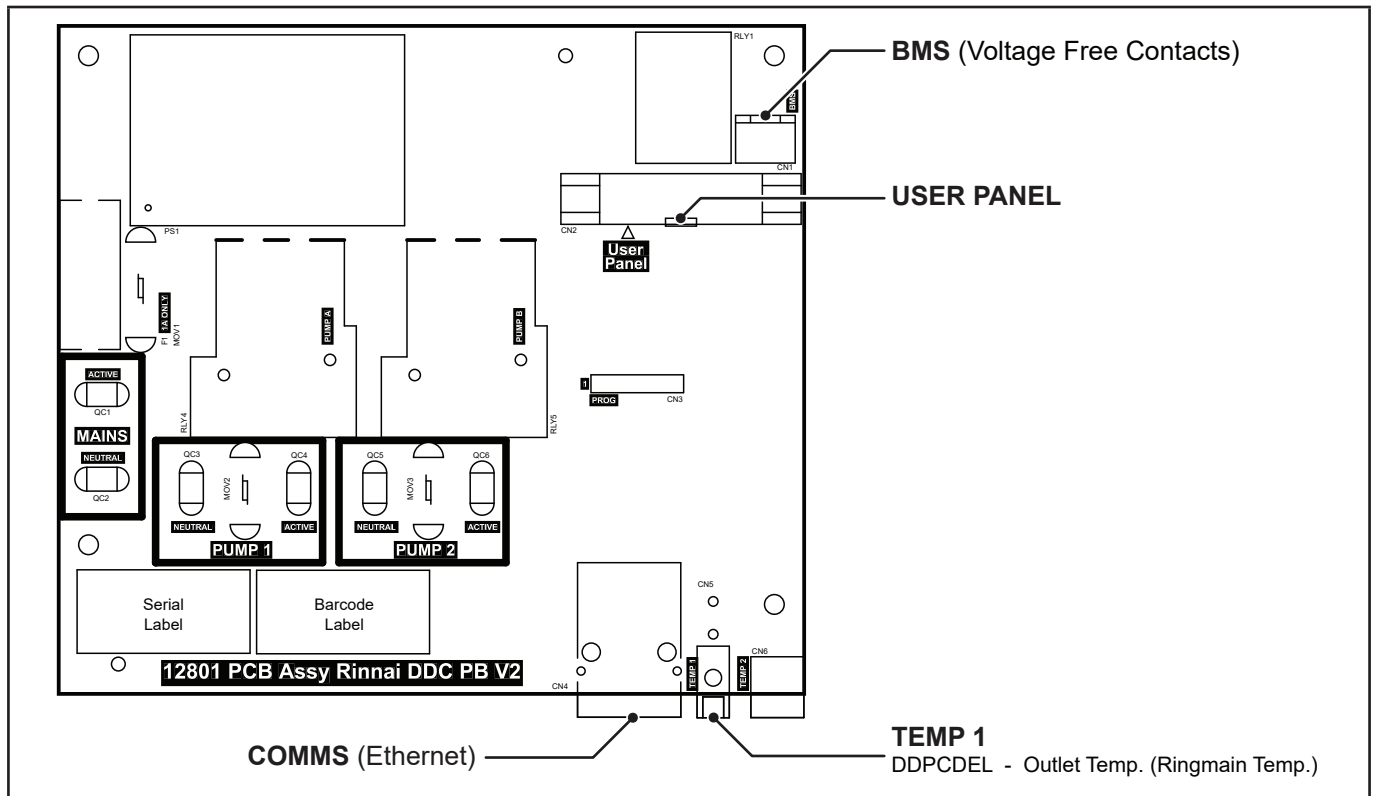
Figure 4. DDPCDEL Internal PCB showing Thermistor Connections
