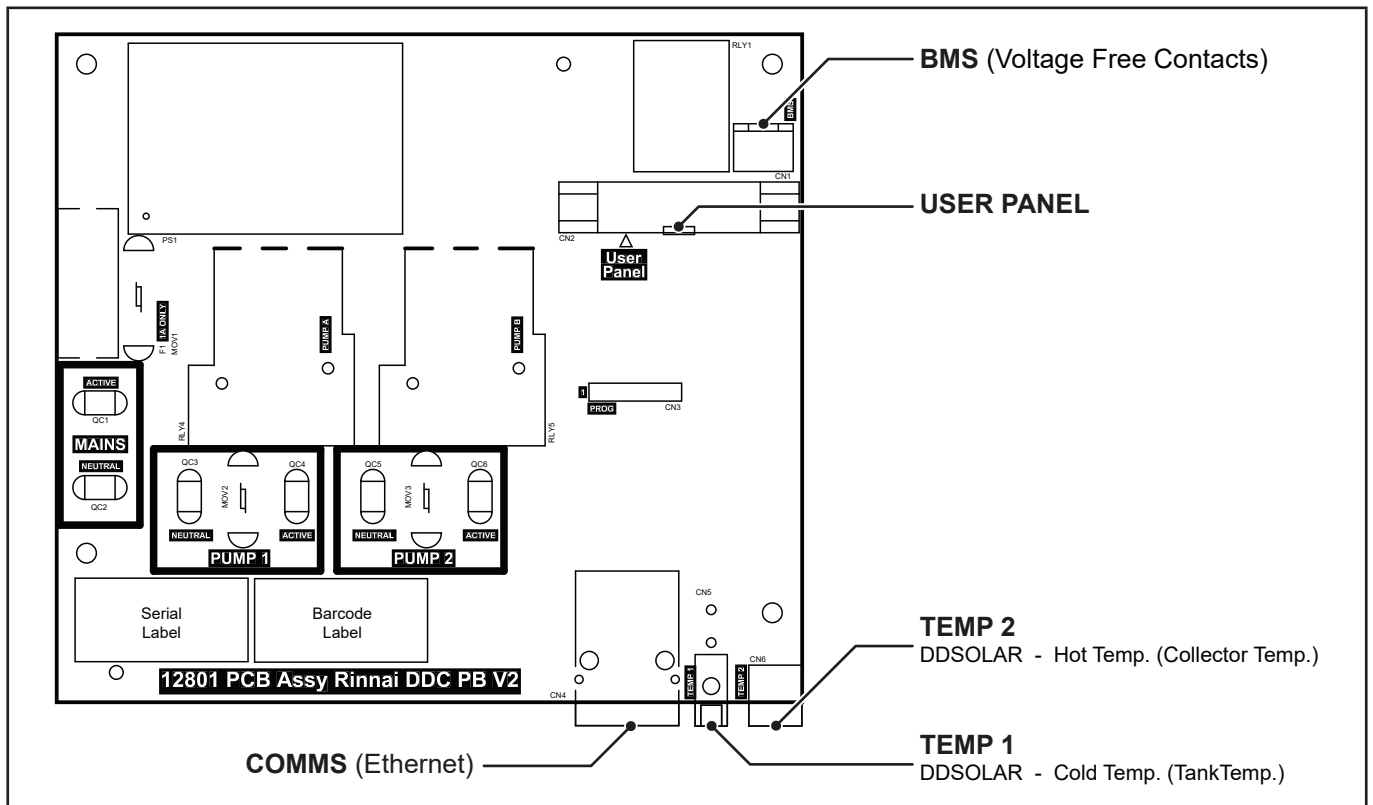
Figure 3. DDSOLAR Internal PCB showing Thermistor Connections
